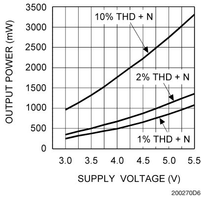
Output Power vs Supply Voltage R_L = 4\Omega + 33\mu H, f = 1\text{kHz}
