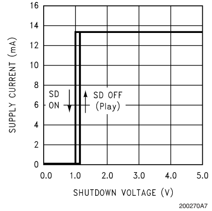
Shutdown Hysteresis Voltage V_{DD} = 5V, \text{SD Mode} = \text{GND (SD High)}
