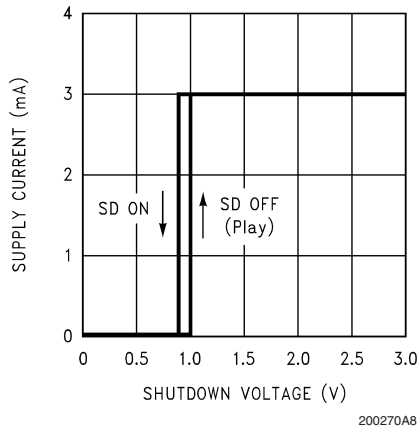
Shutdown Hysteresis Voltage V_{DD} = 3V, \text{SD Mode} = \text{GND (SD Low)}
